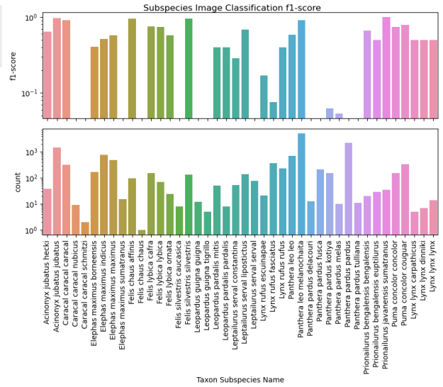
(b) Image-model Taxon Subspecies Performance
