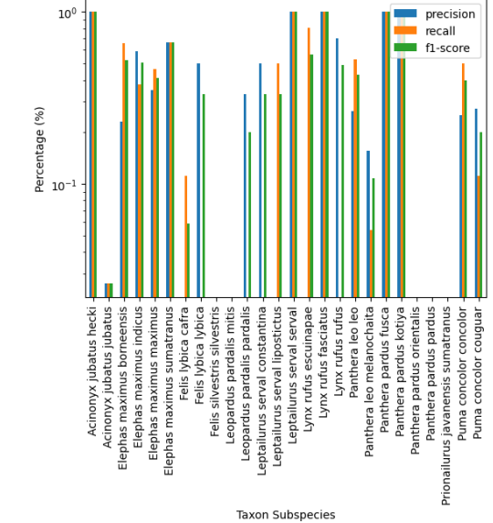
(d) Performance Differences between the Cascading Ensemble Classifier and the Image Classifier at the Subspecies Taxonomy
