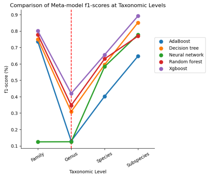
Fig. 8: Metadata Model f1-score per Taxonomic Level
