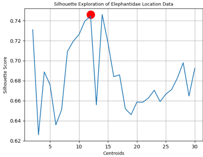
(b) Silhouette Score for Centroid Range with Global Maximum Score
