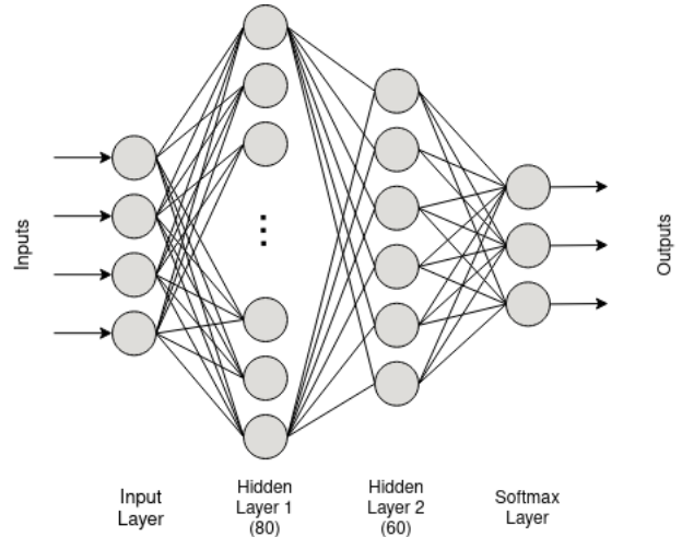
Fig. 4: Neural Network Metadata Model Architecture
