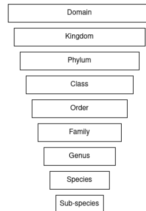
Fig. 1: Taxonomic Classification
