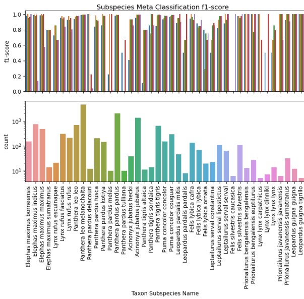
(a) Metadata-model Taxon Subspecies Performance
