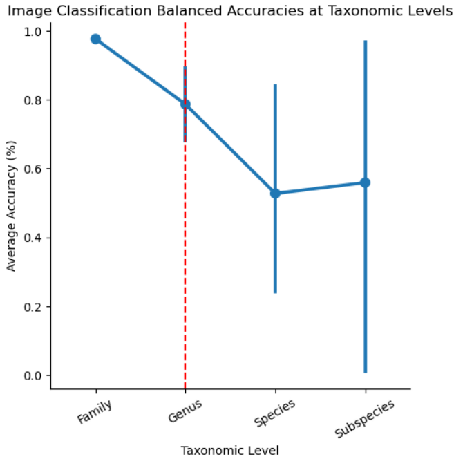
Fig. 9: Average Balanced Accuracy Image Classification Performance per Taxonomic Level
